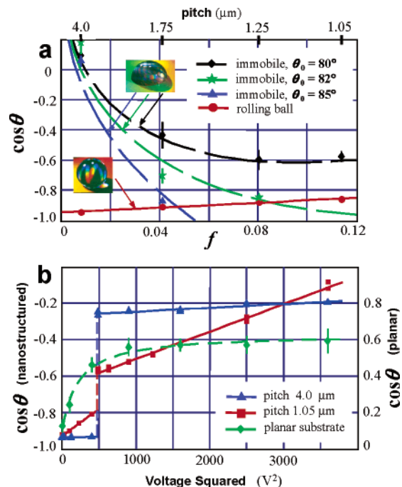
Figure 3. Contact angle \theta of the droplet as a function of the applied voltage and the areal density of nanostips f . (a) \cos \theta as a function of f for 30, 40, and 50% methanol–water mixtures (contact angle on the planar substrate \theta_0 = 85, 82, and 80^\circ ). The rolling ball states are shown as one curve because of the scale of the figure. The red line represents the best linear fit, while the blue, green, and black lines are to guide the eye only. The vertical lines represent standard deviation. (b) \cos \theta as a function of applied voltage squared for the molten salt on the nanostructured and planar substrates. The solid lines represent the best linear fit, while the dashed lines are to guide the eye only. The vertical lines represent standard deviation.
