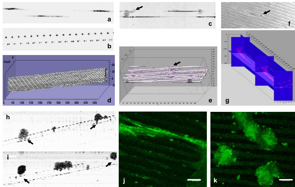
Fig. 6 OCT imaging of cell-substrate interactions. 2-D (a-c) and 3-D (d) OCT images of microtextured (microgrooved) PDMS substrates used for cell culture (e,g,h,i). OCT images (a-e, g-i) were compared with corresponding phase contrast (f) and fluorescence microscopy (j,k) images. Individual cells are indicated by arrows. Mechanical effects on cell-substrate interactions are visualized (h-k). Images are also shown before (h,j) and after (i,k) 5% equibiaxial stretching. Scale bar represents 80 \mu\text{m} .
