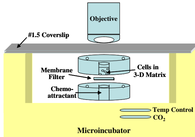
Fig. 1. Experimental set-up for cell chemotactic migration studies. A modified Boyden chamber is shown, in expanded view to show membrane filter, and contained with a microincubator chamber for long-term imaging studies on a microscope stage.
