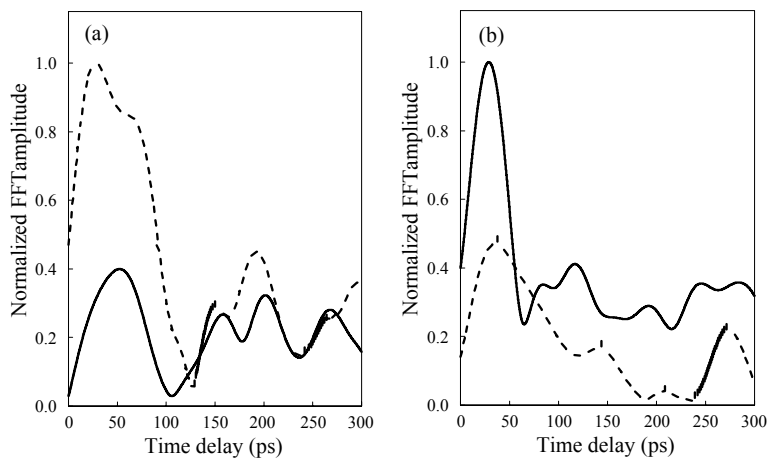
Fig. 1. Variation with time delay of the Fourier amplitude of the 608 cm -1 (solid curve) and 70 cm -1 (dashed curve) frequency components of Rb wavepackets. In taking these data, the pump is parallel to the probe, and both are linearly polarized. The Rb number density is (a) 6 × 10 13 cm -3 and (b) 3 × 10 14 cm -3 .
