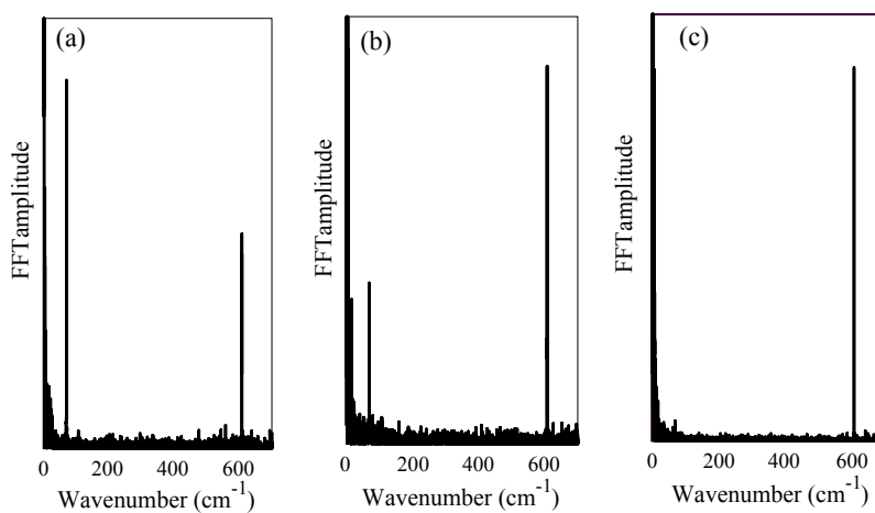
Fig. 2. FFT amplitudes for a fixed Rb number density (6 × 10 13 cm -3 ). The pump is parallel to the probe, and both are linearly polarized. The laser pulse width is 100 fs, the repetition rate is 1 kHz and the total peak intensity of the pump and probe pulses is (a) 2.5 × 10 11 Wcm -2 , (b) 5.5 × 10 11 Wcm -2 and (c) 8.5 × 10 11 Wcm -2 .
