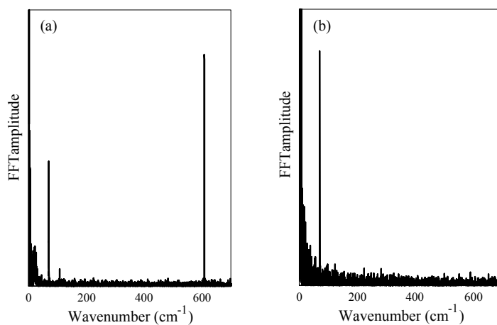
Fig. 3. FFT amplitudes for a fixed Rb density (6 × 10 13 cm -3 ). The total peak intensity of the pump and probe pulses is 2.5 × 10 11 Wcm -2 . (a). The pump is parallel to the probe, and both are linearly polarized. (b). Both the pump and probe are circularly polarized.
