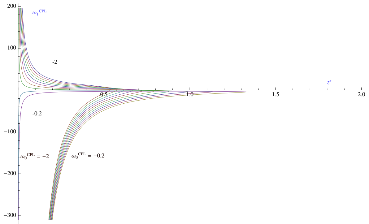
Figure 5: Equation of state linear in a : \omega^{CPL}(z) = \omega_0^{CPL} + \omega_1^{CPL} \frac{z}{1+z} . Plot of \omega_1^{CPL}-z^* for -2 < \omega_0^{CPL} < -0.2 in increments of \Delta\omega_0^{CPL} = 0.2 .
