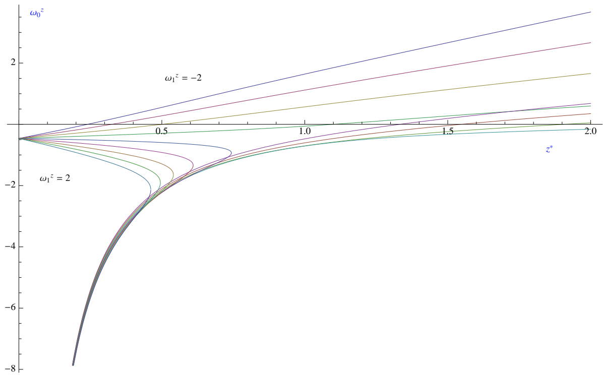
Figure 3: Equation of state linear in z : \omega^z(z) = \omega_0^z + \omega_1^z z . Plot of \omega_0^z - z^* for -2 < \omega_1^z < 2 in increments of \Delta\omega_1^z = 0.5 .
