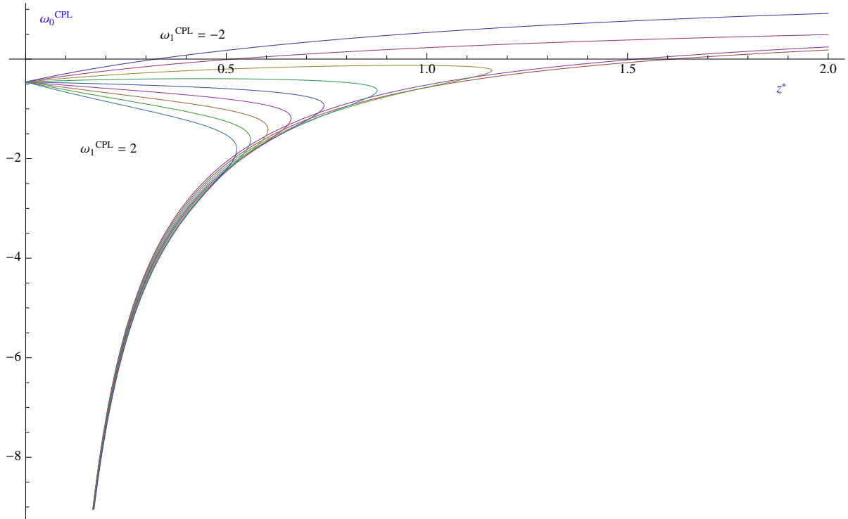
Figure 6: Equation of state linear in a : \omega^{CPL}(z) = \omega_0^{CPL} + \omega_1^{CPL} \frac{z}{1+z} . Plot of \omega_0^{CPL}-z^* for -2 < \omega_1^{CPL} < 2 in increments of \Delta\omega_1^{CPL} = 0.5 .
