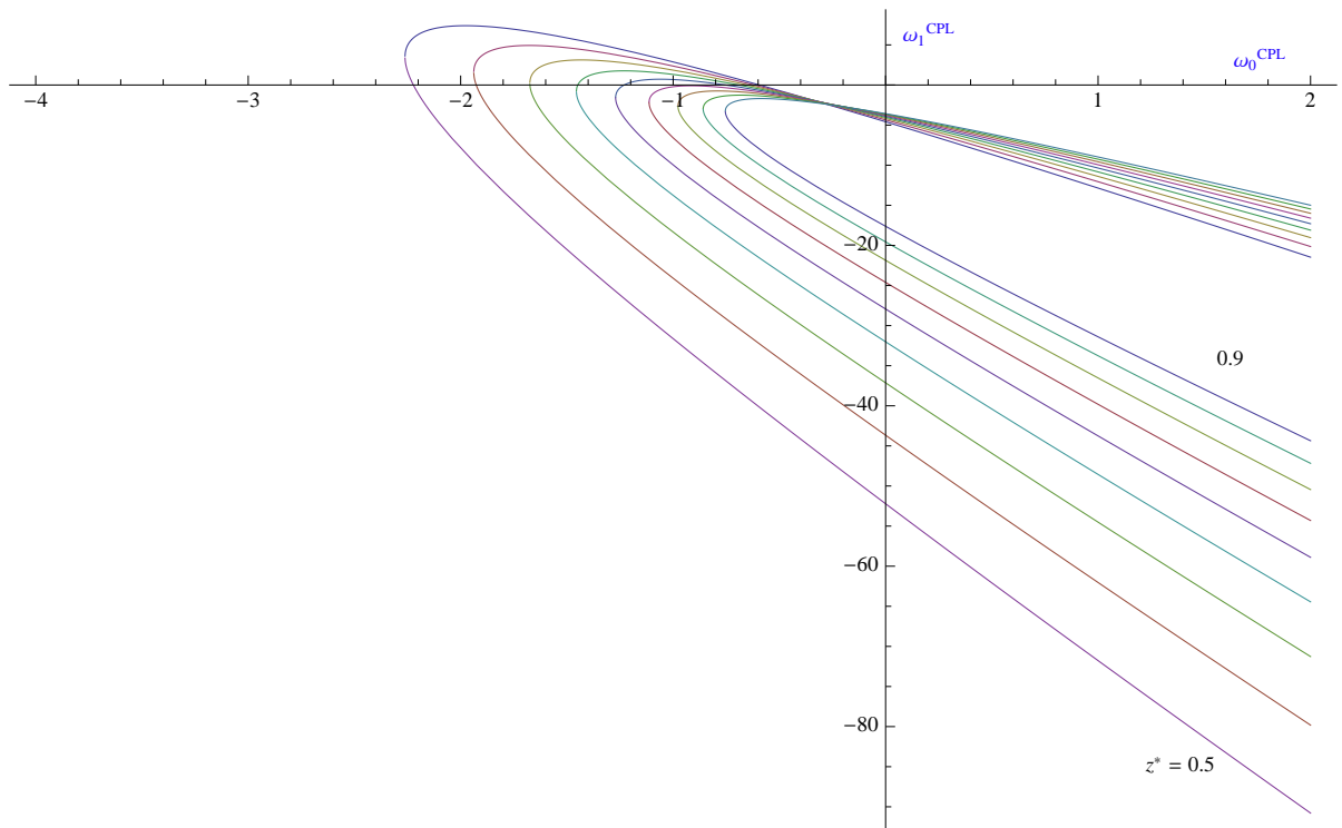
Figure 4: Equation of state linear in a : \omega^{CPL}(z) = \omega_0^{CPL} + \omega_1^{CPL} \frac{z}{1+z} . Plot of \omega_1^{CPL} - \omega_0^{CPL} for 0.5 < z^* < 0.9 in increments of \Delta z^* = 0.05 .
