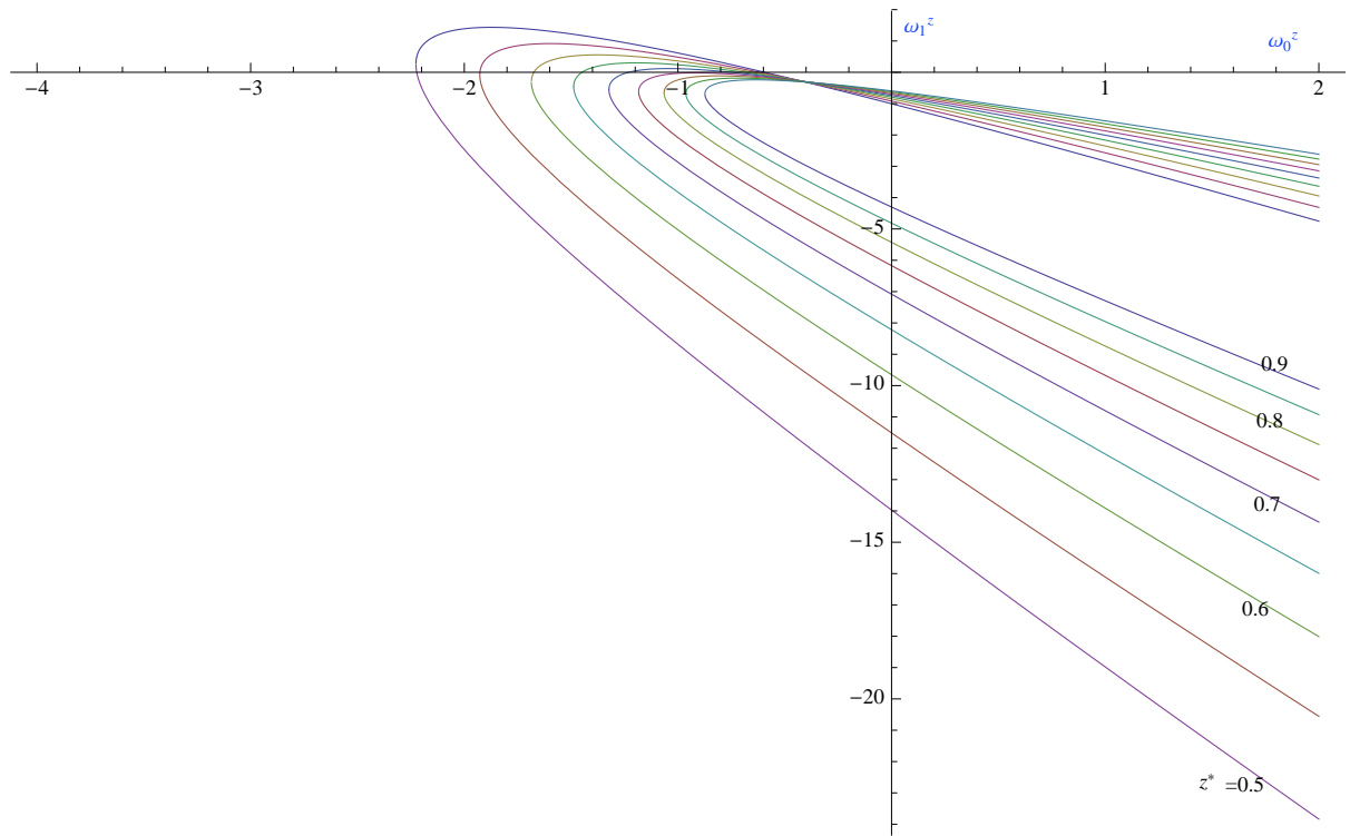
Figure 1: Equation of state linear in z : \omega^z(z) = \omega_0^z + \omega_1^z z . Plot of \omega_1^z - \omega_0^z for 0.5 < z^* < 0.9 in increments of \Delta z^* = 0.05 .
