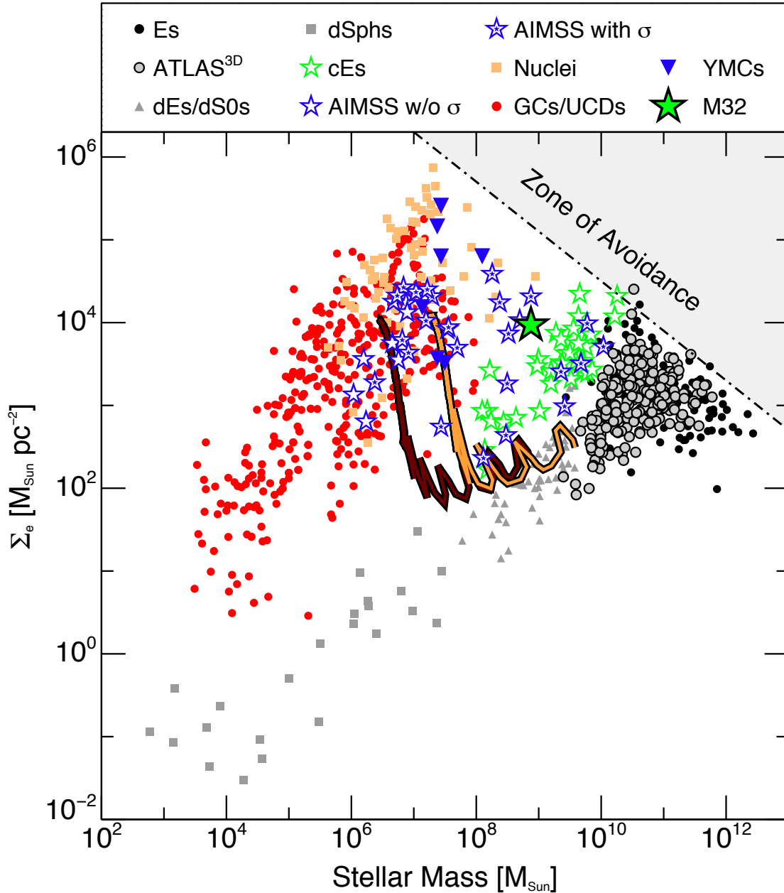
Figure 14. Stellar mass vs. effective stellar mass surface density for dynamically hot stellar systems. Symbols are the same as those defined in Figure 11. The effective stellar mass surface density is calculated as \Sigma_e = M_x / 2\pi R_e^2 . The “zone of avoidance” translated from that shown in Figure 13 is shown by the grey shaded region. The solid orange and brown lines are the same simulations from Pfeffer & Baumgardt (2013) as shown in Figure 13. In this plane it is even clearer that there is a separation between the densest objects discussed here and the majority of the compact stellar system population.
