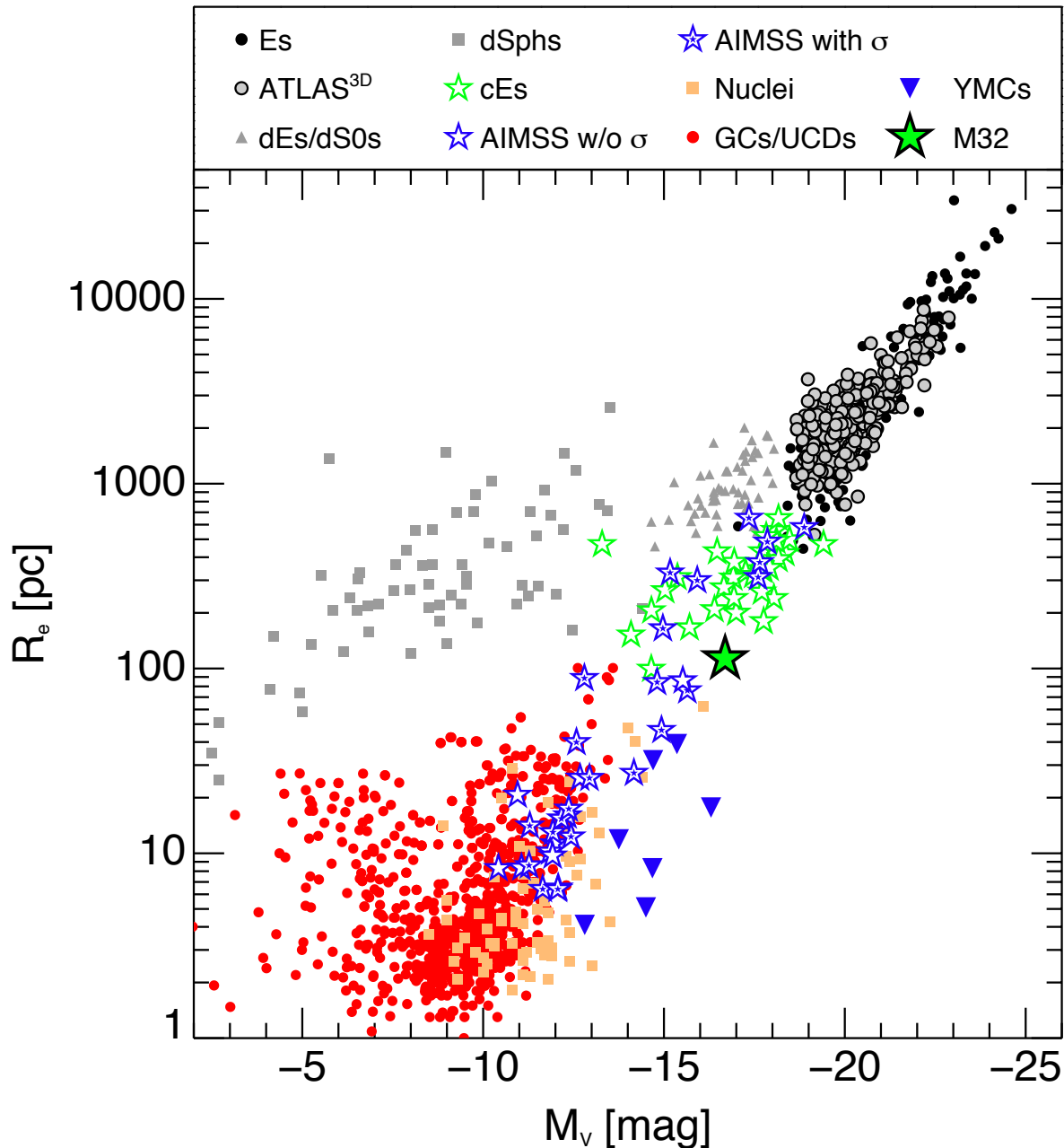
Figure 11. Effective radius R_e vs absolute V-band magnitude M_V for dynamically hot stellar systems from our master compilation. Blue stars are our observations and are filled where we have successfully measured the velocity dispersion of the object. M32 is indicated by its own symbol and labelled. It is clear that the group of six (including one literature Coma cE) non-YMC objects with M_V < -14 and R_e < 100\text{pc} lie offset significantly from the more massive previously known UCDs such as Virgo-UCD7 and Fornax-UCD3, which are smaller than M32.
