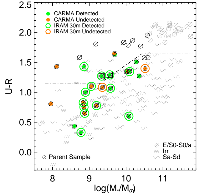
FIG. 1.— U - R color vs. stellar mass for galaxies in the Nearby Field Galaxy Survey (Jansen et al. 2000), plus five additional E/S0s from the literature. Symbols denote morphological types (KGB). The red sequence, i.e. the main locus of traditional red E/S0s, lies above the dashed line (with two borderline “mid-sequence” E/S0s boxed, see KGB), while the blue sequence (typically populated by spirals) lies below. Dark symbols denote the 32 galaxies in the parent sample; the rest of the NFGS is shown in light grey.
