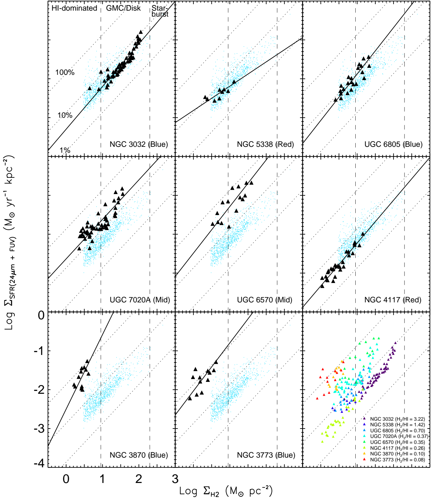
FIG. 2.— \Sigma_{\text{SFR}} vs. \Sigma_{\text{H}_2} at 750 pc resolution. Points for the seven spirals from Bigiel et al. (2008) are plotted in light blue. Black triangles show our eight E/SOs resolved in CO(1–0) with CARMA. Vertical dashed lines demarcate the three different regimes of star formation discussed in Bigiel et al. (2008), and dotted lines mark constant MSFE, corresponding (from top to bottom) to the depletion of 100%, 10%, and 1% of the molecular gas (including helium) within 10^8 yr, or equivalently to molecular gas depletion timescales of 0.1, 1, and 10 Gyr. Solid black lines represent OLS bisector fits. The color sequence (blue/mid/red) is noted at the bottom of each panel. The last panel combines the points for all eight galaxies, color-coded by M_{\text{H}_2}/M_{\text{HI}} , illustrating variations in MSFE with power-law index N and M_{\text{H}_2}/M_{\text{HI}} (see §3 and §5).
