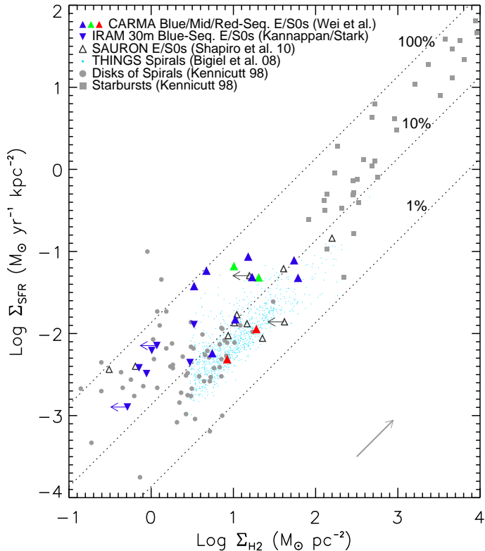
FIG. 3.— Aperture-averaged \Sigma_{\text{SFR}} vs. \Sigma_{\text{H}_2} for normal disk and nuclear starburst galaxies from Kennicutt (1998), SAURON E/SOs from Shapiro et al. (2010), and E/SOs from this Letter. The 750 pc resolution points from Bigiel et al. (2008) are also plotted in the background for comparison. Dotted lines mark the same lines of constant MSFE as in Figure 2. Grey arrow in the lower right shows typical shift of spiral disk points from Kennicutt (1998) if averaged over 0.6 R_{25} instead of R_{25} .
