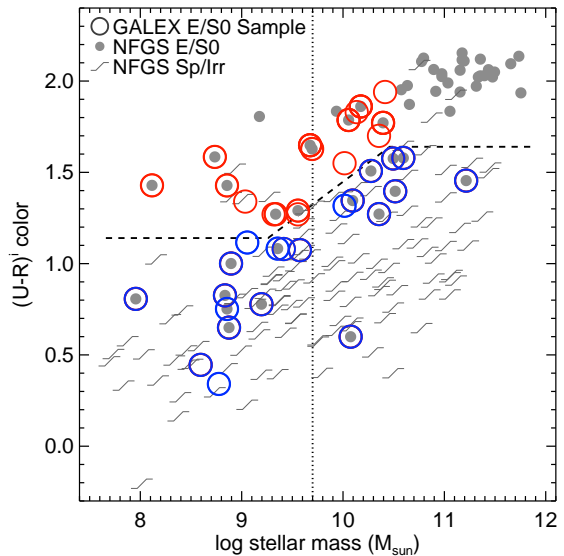
Figure 1. GALEX GI and archival E/SO sample in color-stellar mass space. The small grey symbols indicate galaxies in the Nearby Field Galaxy Survey, the parent sample for the majority of our E/SOs (§2). The dashed line divides the red and blue sequences, and the vertical line marks the gas-richness threshold mass (KGB). The 38 E/SOs with GALEX data are denoted by open circles.
