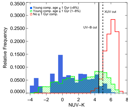
Figure 4. NUV-K color for selected composite stellar population models (grid as described in §3.2.1), illustrating NUV-K cuts chosen for our analysis. Blue and green histograms represent numbers of models with >8\% and 1-8\% young population contributions by mass, normalized to the total numbers of such models. The red histogram represents numbers of models containing no young (age \leq 1 Gyr) component, normalized to the total numbers of such models. It is apparent that the fraction of purely old models increases significantly beyond NUV-K = 5 , so we use this value to reject XUV disks likely to contain evolved populations as described in §3.2.1. A more conservative color cut at NUV-K = 4.5 appears necessary if we wish to select populations with a significant young population as in our UV-B disk classification (here >8\% , corresponding to the \gtrsim 10\% requirement specified in §3.3).
