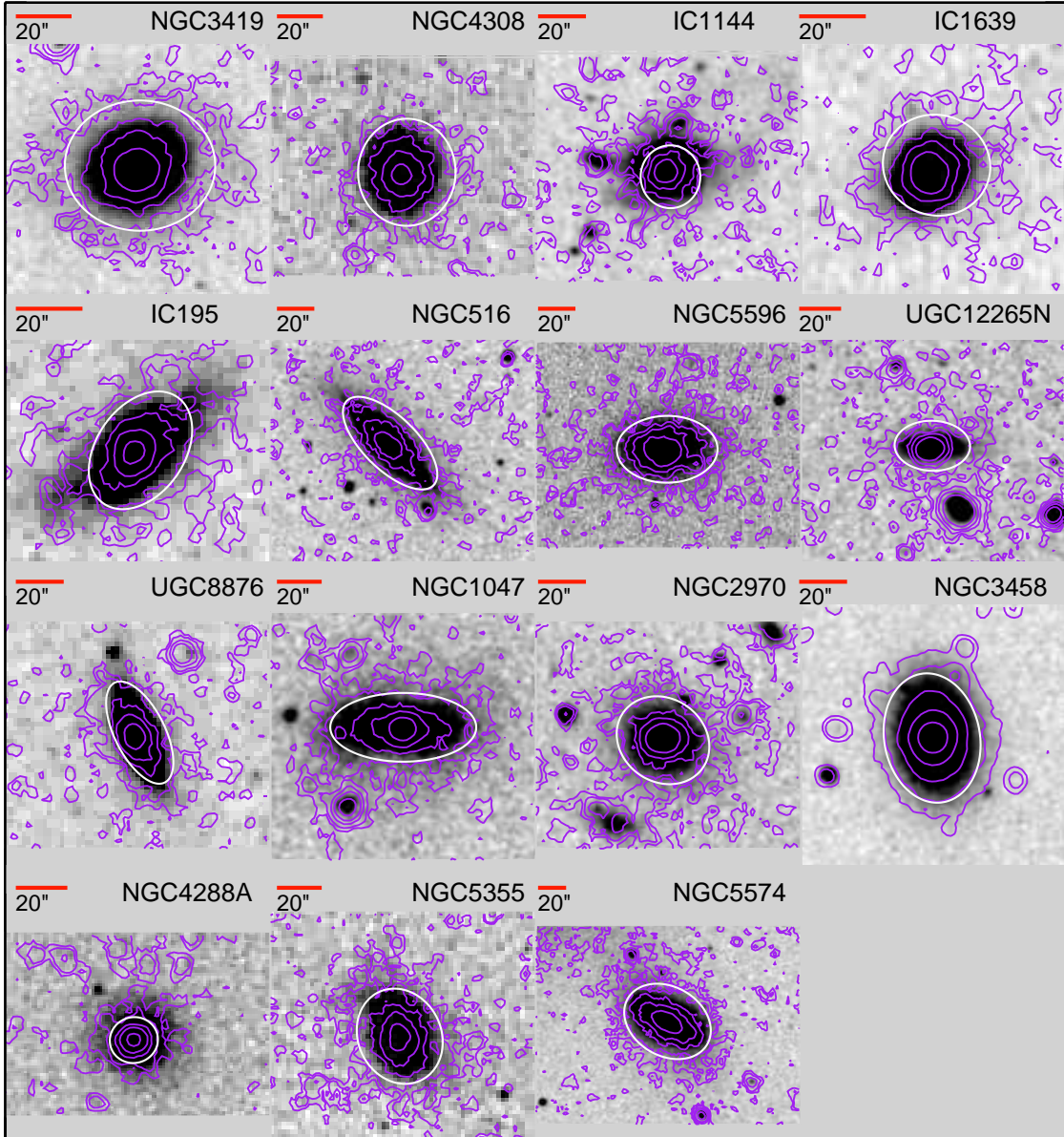
Figure 10. Smoothed NUV contours (purple) overlaid on DSS-II red images of E/S0s in our sample without XUV or UV-B disks. R_{UVSF} is indicated in white, and contours start at \sim 28.6 AB mag arcsec ^{-2} and go up by 2\times , 5\times , 10\times , and 25\times in intensity. Five of these are Type 1 XUVs by the T07 definition: NGC3419, NGC4308, IC195, UGC8876, and NGC5355. Some galaxies where the contours show extent beyond R_{UVSF} do not pass the test that this emission is >3\sigma above the PSF shelf (see §3.2.2).
