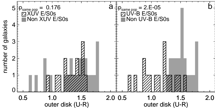
Figure 6. Optical outer-disk colors for sample E/S0s, calculated between the 50%–75% B -band light radii for NFGS E/S0s and between the 50%–75% g -band light radii for all others ( u-r color is used as a proxy for U-R for non-NFGS galaxies, with a shift to U-R color as applied in KGB). (a) Comparison of E/S0s with and without XUV disks, illustrating that XUV-disk E/S0s do not show bluer optical outer-disk colors than E/S0s without XUV disks, i.e., do not show enhanced outer-disk star formation. (b) Comparison of E/S0s with and without UV-B disks, illustrating that UV-B disk E/S0s do show bluer optical outer-disk colors than E/S0s without UV-B disks, i.e., do show clearly enhanced outer-disk star formation.
