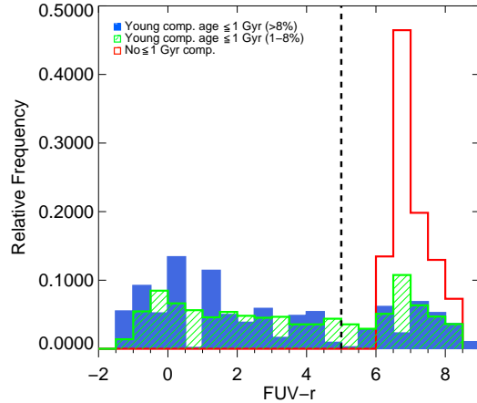
Figure 3. FUV-r color for selected composite stellar population models (grid as described in §3.2.1), illustrating issues with using this color as a clean young/old population divider. Blue and green histograms represent numbers of models with >8\% and 1-8\% young population contributions by mass, normalized to the total numbers of such models. The red histogram represents numbers of models containing no young (age \leq 1 Gyr) component, normalized to the total numbers of such models. The vertical dashed line indicates the color cut of Lemonias et al. (2011), which appears to miss a significant fraction ( \sim 30\% ) of the combined young model options that fall outside this cut with colors redder than FUV-r = 5 .
