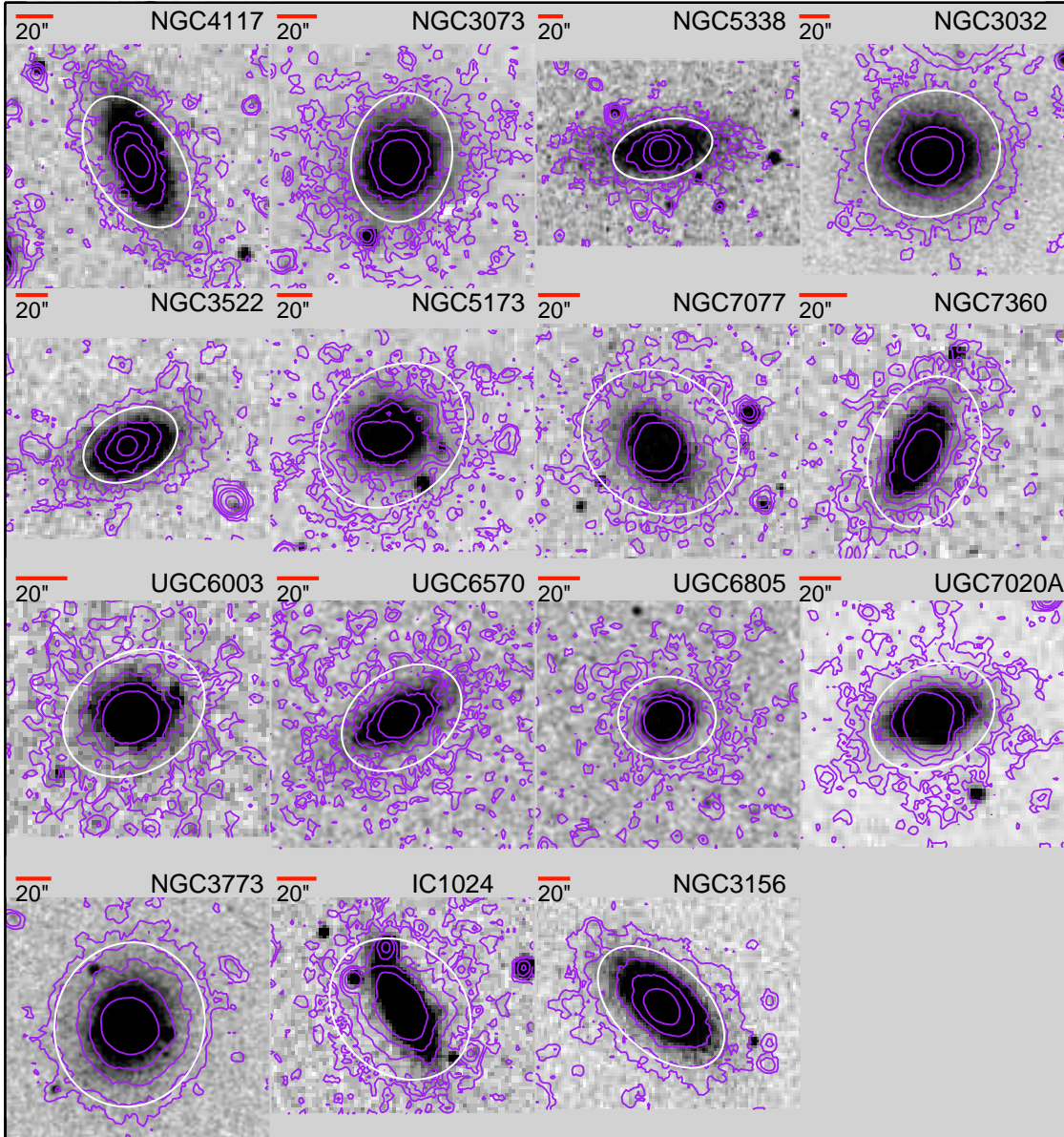
Figure 8. Smoothed NUV contours (purple) overlaid on DSS-II red images of XUV-disk E/S0s. R_{\text{UVSF}} is indicated in white, and contours start at \sim 28.6 AB mag arcsec ^{-2} and go up by 2\times , 5\times , 10\times , and 25\times in intensity. Eleven of these are Type 1 XUVs by the T07 definition: NGC4117, NGC3073, NGC5338, NGC3522, NGC5173, NGC7077, NGC7360, UGC6003, UGC7020A, IC1024, and NGC3156. Eight of these are also UV-Bs: NGC3073, NGC5173, NGC7077, UGC6003, UGC6805, UGC7020A, NGC3773, and IC1024.
