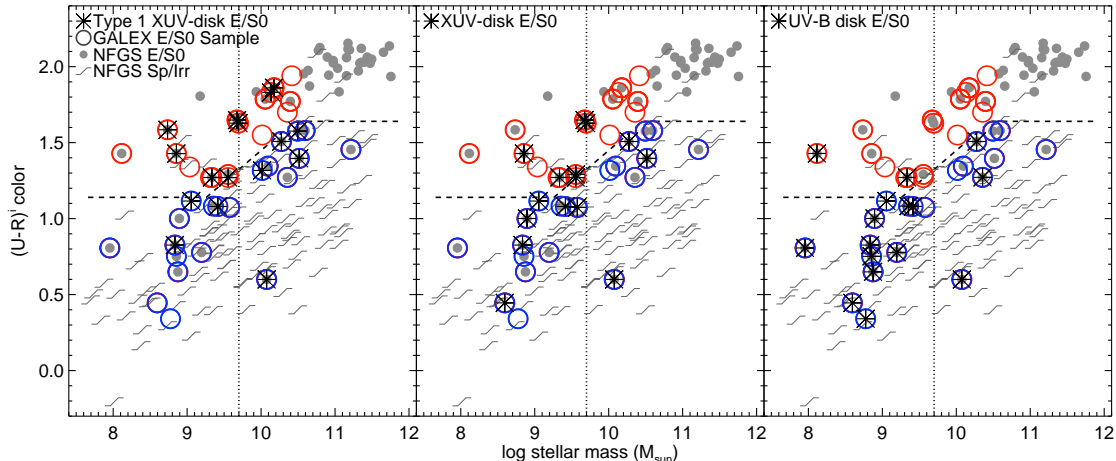
Figure 5. GALEX GI and archival E/S0 sample in color–stellar mass space (as in Figure 1), showing UV disks (asterisks) identified according to three different classifications: (left) the original T07 XUV-disk definition, (middle) our new, purely quantitative XUV definition, and (right) the UV-B disk definition.
