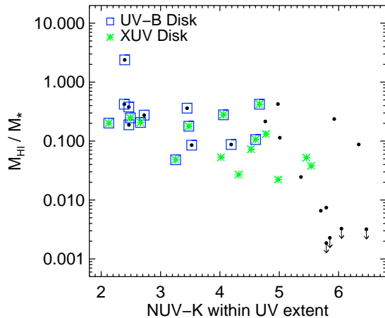
Figure 7. HI content versus NUV-K color measured within the detected NUV extent, illustrating the trend towards enhanced HI content in UV-B disk galaxies (blue squares). Black points represent all sample galaxies with HI data ( M_{HI} from references noted in Table 2), and green stars represent XUV disks. Note that the plotted NUV-K colors are not those used for classification of either XUV or UV-B disks.
